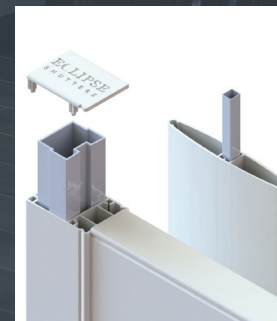
Aluminum Reinforcement
